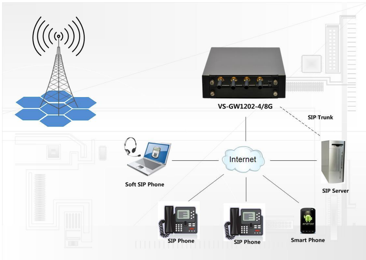
Figure 1-2-1 Topological Graph
