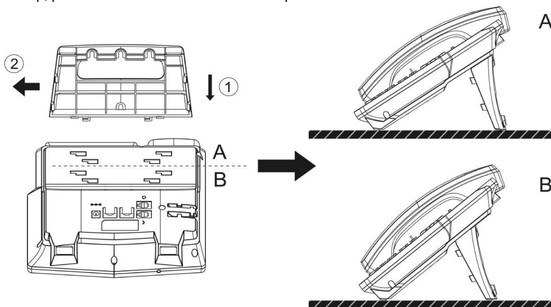
Figure 1 - Desktop Installation
