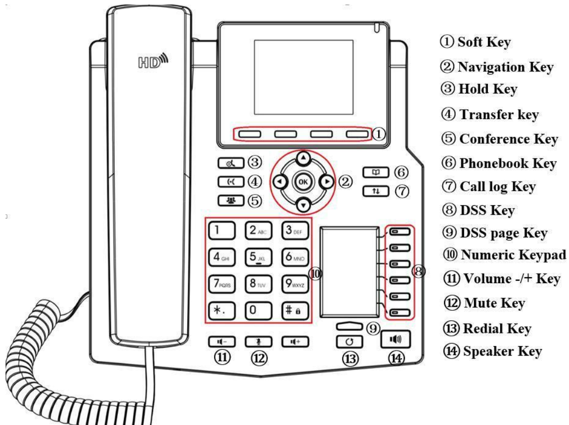
Figure 4 - Keypad
