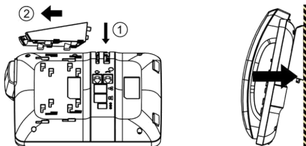
Figure 2 - Wall-mount Installation
