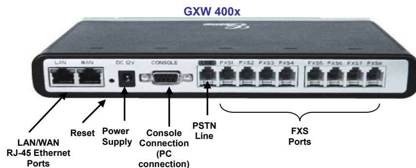
Figure 1: Diagram of GXW4004-8 back panel
