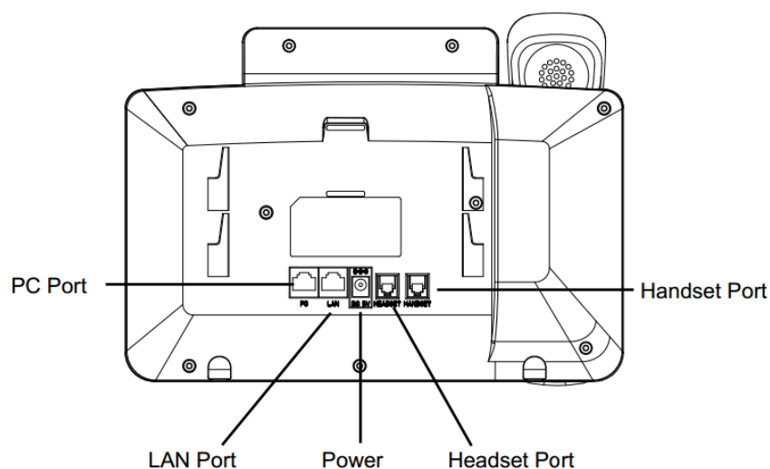
Figure 1: GXP2124 Ports
