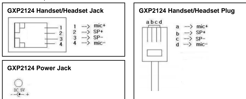
Figure 2: GXP2124 Pin-out
